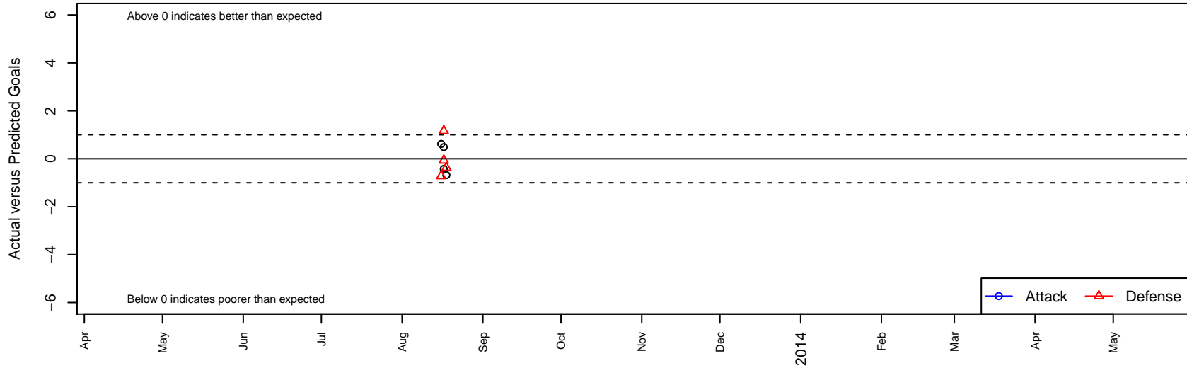
FSC Falcons B01 Dots are actual minus expected GF (blue circles) and GA (red triangles). Blue line is smoothed change in attack strength. Red is smoothed change in defense strength.
